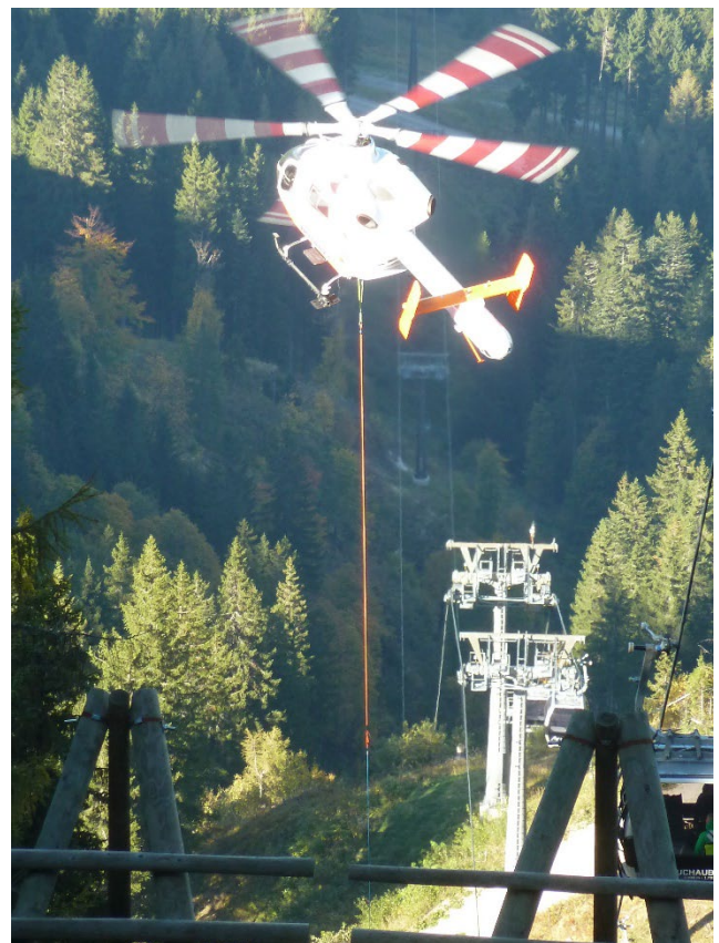
Fig. 2: High visibility with orange fixed rope, manufactured by A&H EQU
